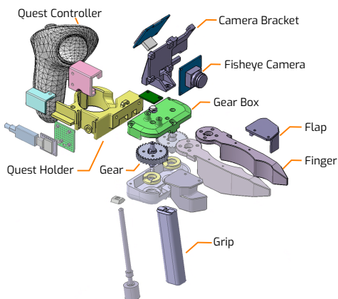
Fig. 3. Exploded view of the YUBI gripper: The bidigital mechanism utilizes internal gears to actuate the jaws, all supported by an ergonomic grip and flap. A fisheye camera is attached for task observation. The Quest controller is integrated to provide high-frequency 6-DoF trajectory tracking.
