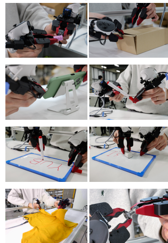
Fig. 2. Overview: To ensure massive, high-quality robot manipulation data for scalable robot learning, we collect bimanual YUBI-based demonstrations at 20 desks in parallel from 104 operators. Our operation setups feature (i) a stereo top-view camera for stable workspace observation, (ii) a rig-mounted VR system for 6DoF gripper tracking where the VR controllers are attached to the YUBI gripper, and (iii) foot pedal-based action segmentation for hands-free control. The collected dataset features diverse 40 tasks that require various skills including assembling bricks and paper boxes, insertion, writing and erasing, folding clothes, and tightening nuts and bolts.
