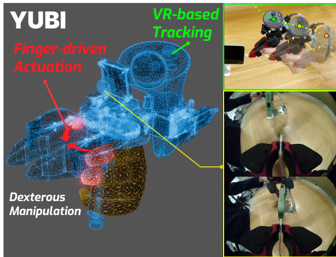
Fig. 1. Yielding Universal Bidigital Interface (YUBI) : Our lightweight, finger-aligned gripper offers intuitive control by mirroring human digital kinematics for dexterous manipulation. Leveraging high-precision VR-based tracking, YUBI facilitates the curation of a large-scale, high-quality bimanual dataset to advance robotic foundation models.
